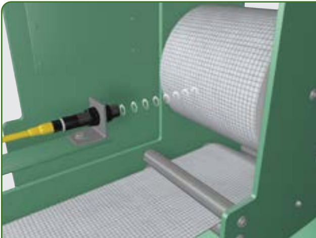
Roll diameter and tank level – An 873P analog ultrasonic continuously measures roll diameter or tank level and provides a proportional 4...20 mA or 0...10V DC output. If a dual discrete output sensor is used, one switch point is set for low level indication and the other set for a full condition.
