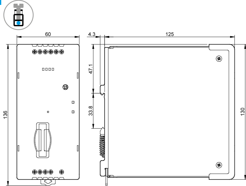
Type 78.2E Screw terminal
