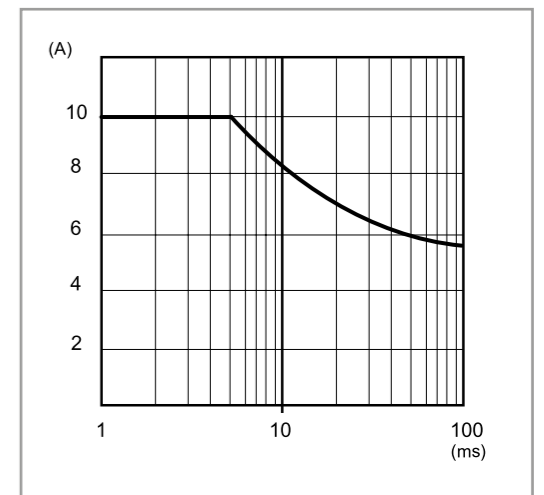
P78-7 Output peak current v time (78.1A)
