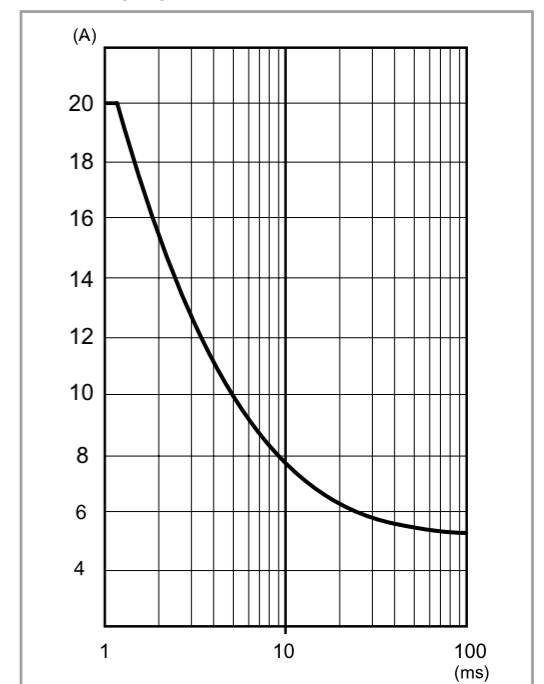
P78-9 Output peak current v time (78.1D)
