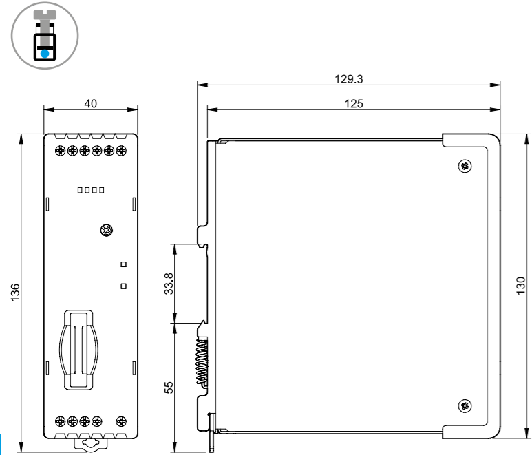
Type 78.1D Screw terminal
