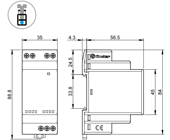
Type 78.25 Screw terminal
