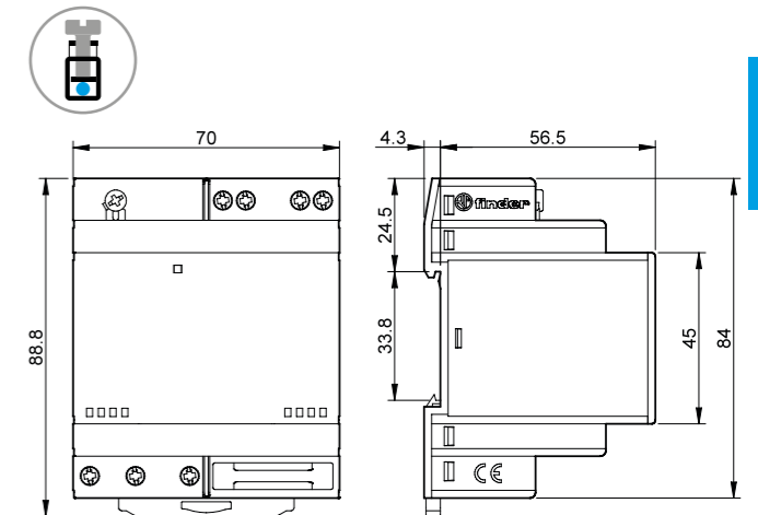
Type 78.1B Screw terminal
