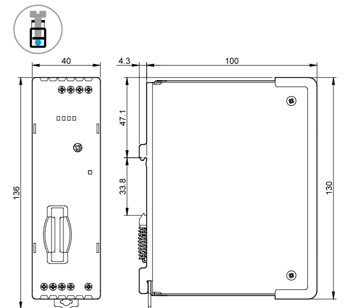
Type 78.1B Screw terminal
