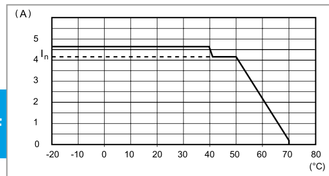
L78-5 Output current v ambient temperature (78.50/51)
