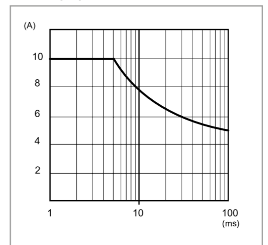
P78-9 Output peak current v time (78.1D)
