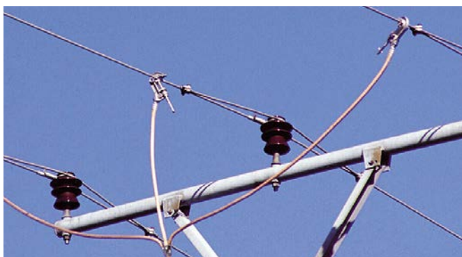
Phase screw clamps used on an overhead line
