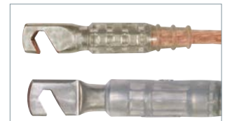
Crimped cable lugs, type PK3: Hook-type cable lugs up to cable cross-sections of 35 mm 2 are available on request.
