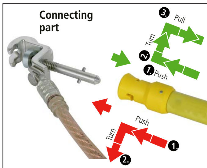
T pin shaft coupling
