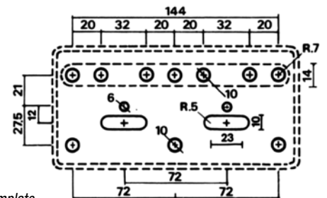
Fixing template
