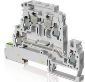
Double deck - For 5 x 20 mm and 5 x 25 mm fuses (0.197" x 0.787" and 0.197" x 0.984")
