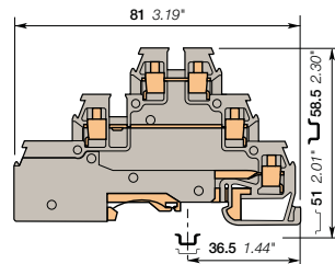
6 mm 0.236 in spacing
